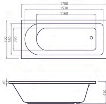
Bath height 410mm (exc. feet)
