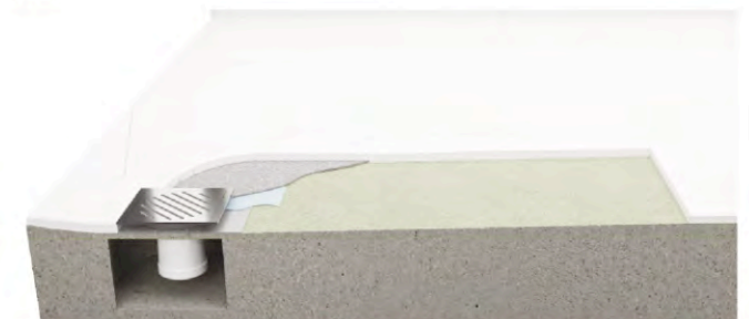
Square drain only creating a channel for the trap and waste pipe.
